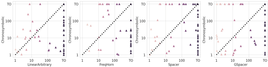
Fig. 4. Running time comparison of CHRONOSYMBOLIC LEARNING and baselines, where the timeout (TO) is 360s. The points below the diagonal indicate instances on which Chronosymbolic-single outperforms baselines. Here, we only plot non-trivial instances (i.e., solving time takes \geq 1 second for both solvers).
